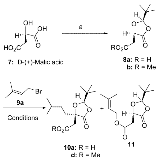
Scheme 4. Reagents: a) 1.7 equiv. pivalaldehyde, cat. p TsOH, cat. \text{H}_2\text{SO}_4 , pentane, reflux, 92%.
