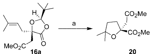
Scheme 9. Reagents: a) 50% \text{H}_2\text{SO}_4 , MeOH, 60 °C, 6 h, 79%.
