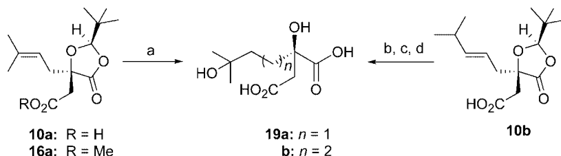
Scheme 8. Reagents: a) i. \text{Hg}(\text{OAc})_2 , NaOH, THF/ \text{H}_2\text{O} (1:5) 5 h, ii. \text{NaBH}_4 , NaOH, room temp., 12 h, 86%; b) \text{SeO}_2 , t\text{BuO}_2\text{H} ; c) \text{H}_2 , \text{PtO}_2 , EtOAc; d) 50% \text{H}_2\text{SO}_4 , dioxane, 60 °C, 6 h, 44% over three steps.
