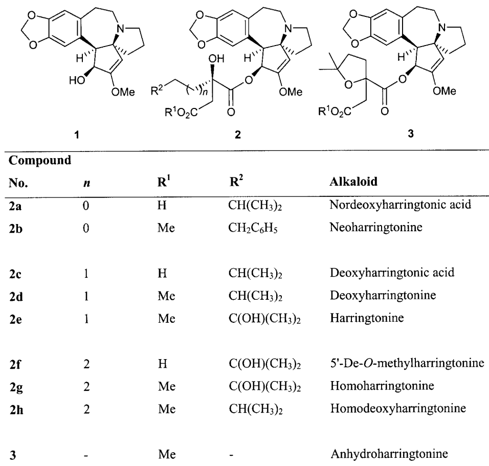
Scheme 1. Cephalotaxus alkaloids.
