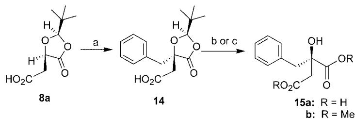
Scheme 6. Reagents: a) 2 equiv. LiHMDS, THF/hexane, –78 °C, 1 h, then benzyl bromide, 87%; b) 50% \text{H}_2\text{SO}_4 , dioxane (1:5), 60 °C, 24 h; c) 50% \text{H}_2\text{SO}_4 , MeOH, 60 °C, 6 h.
