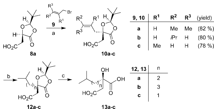
Scheme 5. Reagents: a) 2 equiv. LiHMDS, THF/hexane –78 °C, 1 h, then 9 ; b) \text{H}_2 , \text{PtO}_2 , EtOAc; c) 50% \text{H}_2\text{SO}_4 , dioxane (1:5), 60 °C, 24 h.
